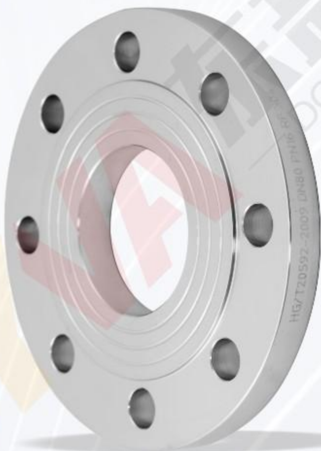
平焊法兰 Flat welding flange
