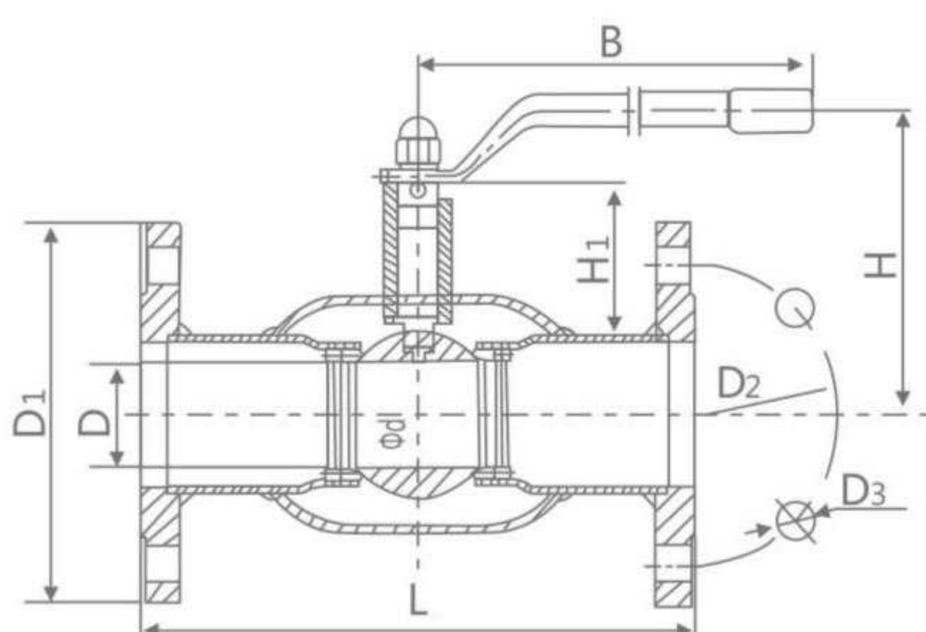
缩径/法兰 Shrinkage/Flange
