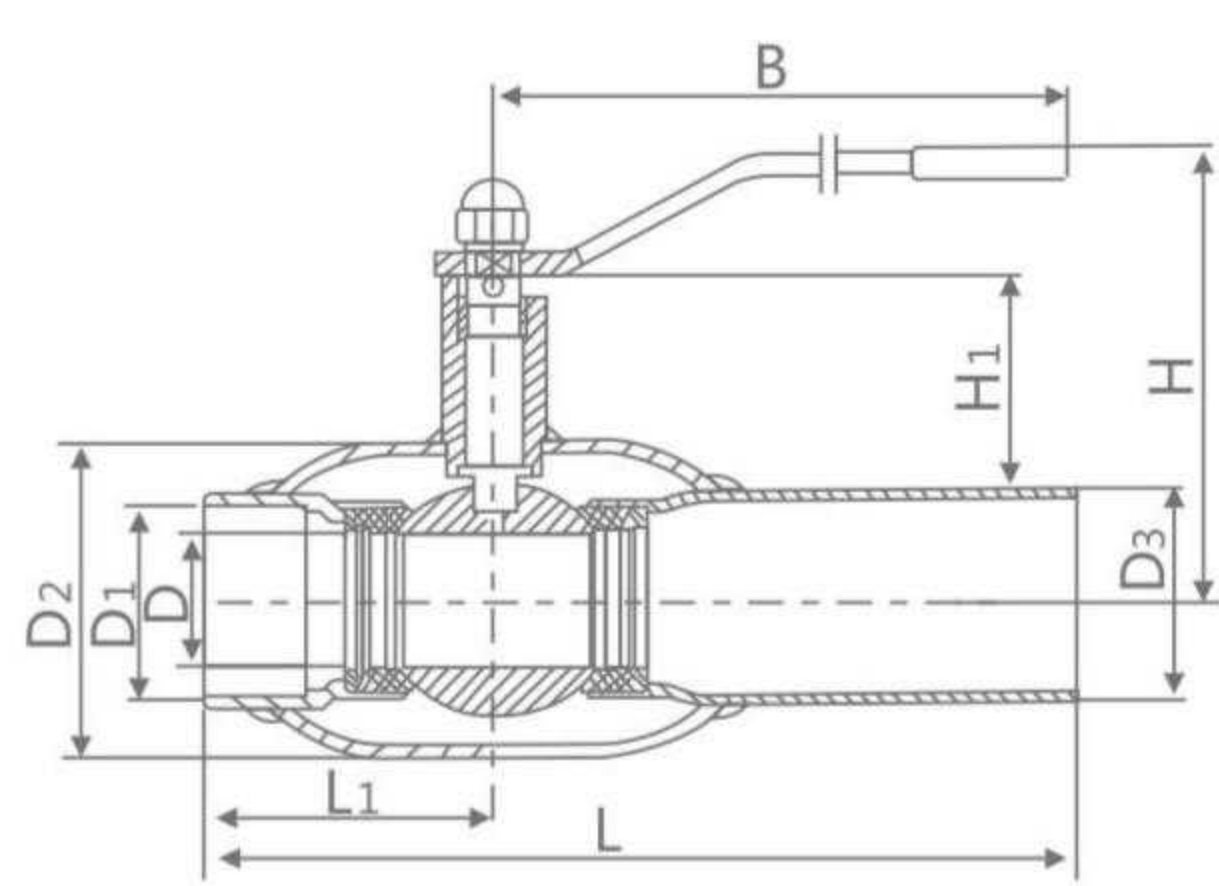
缩径/螺纹&焊接 Shrinkage/Screw & Welding
