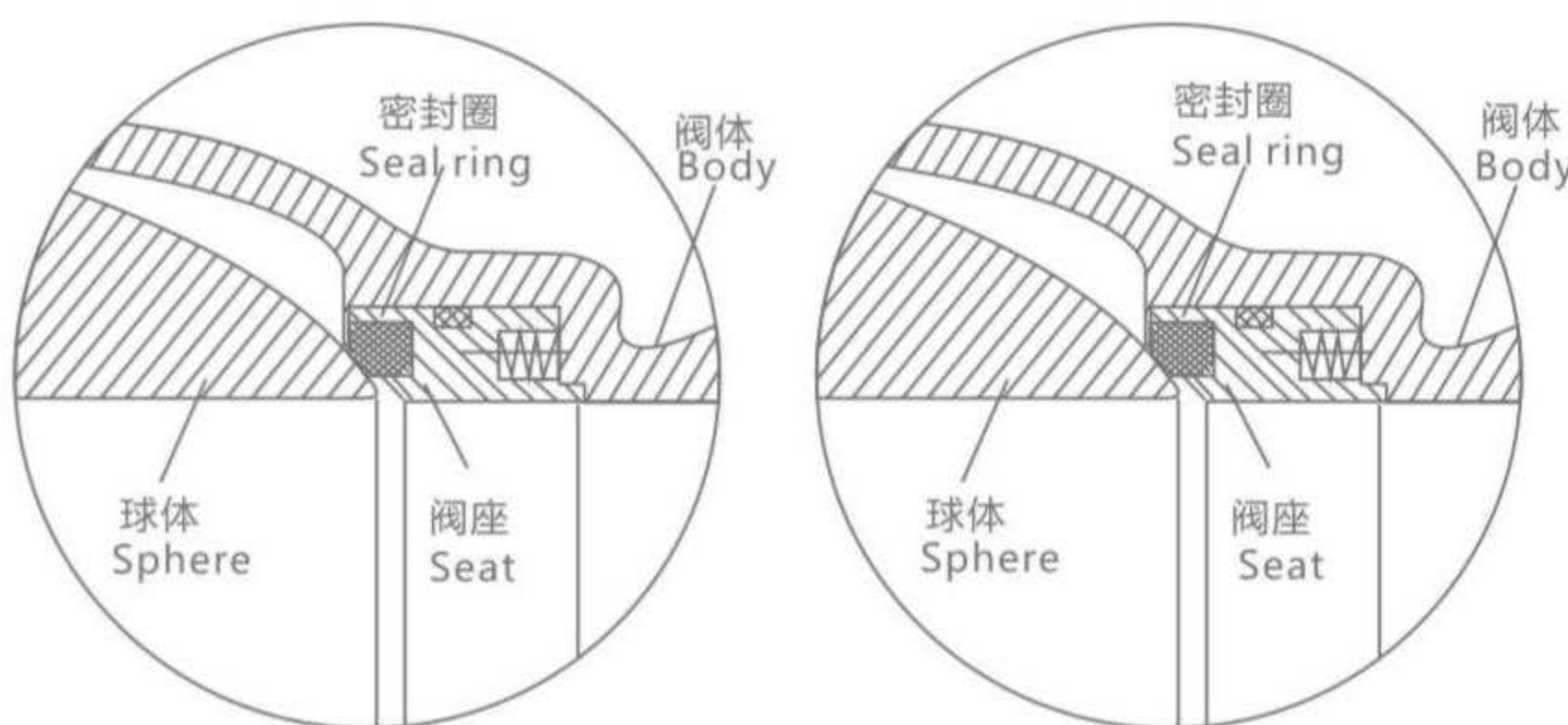
平常时的密封 Usual seals when 软密封烧损时的密封 Burning of soft seal when the seal
