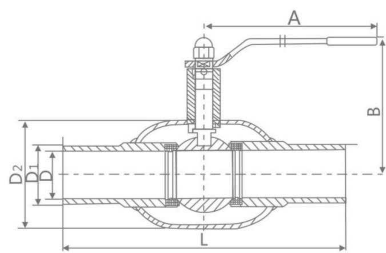
全径/焊接 Full diameter/Welding
